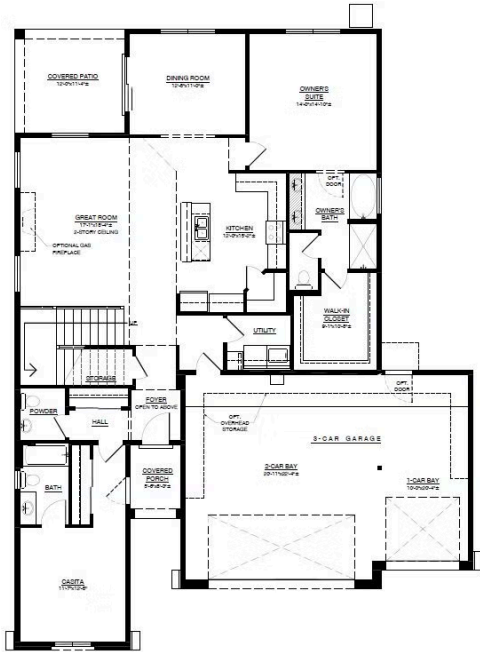
FIRST FLOOR W/OPT. CASITA & OPT. 3-CAR GARAGE
