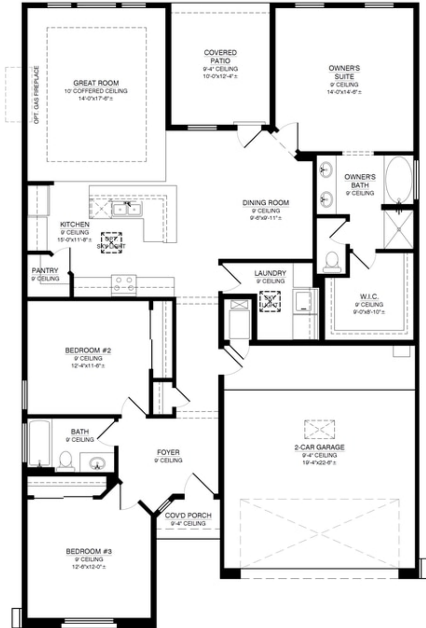
FLOOR PLAN
