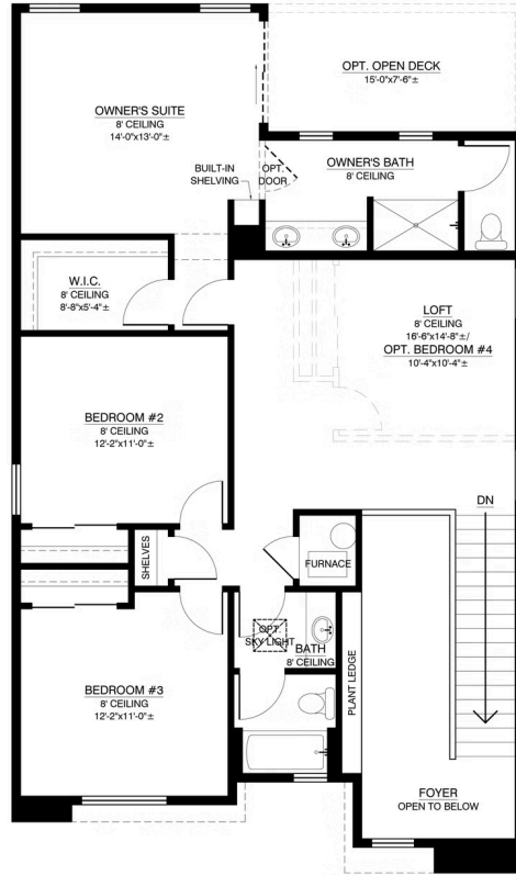
2ND FLOOR
