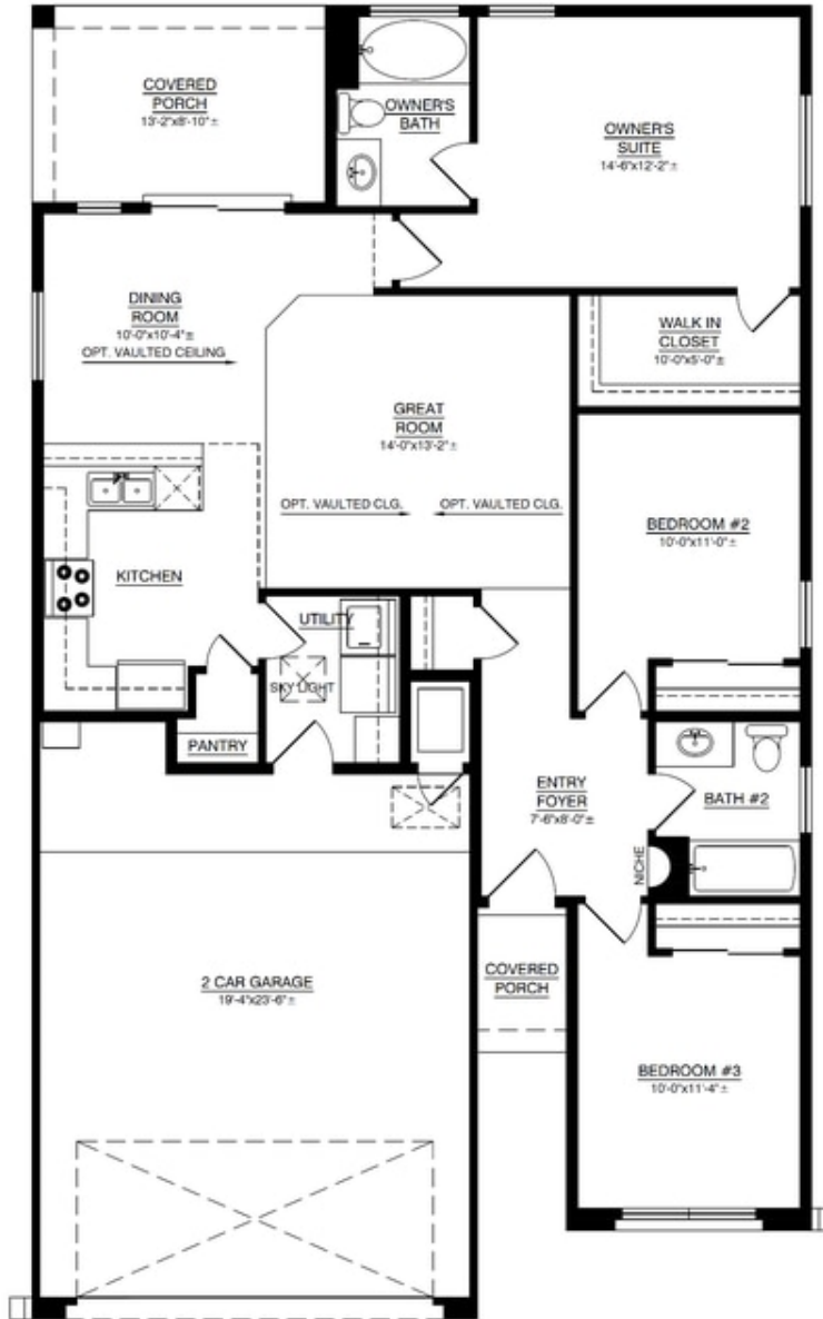
FLOOR PLAN
