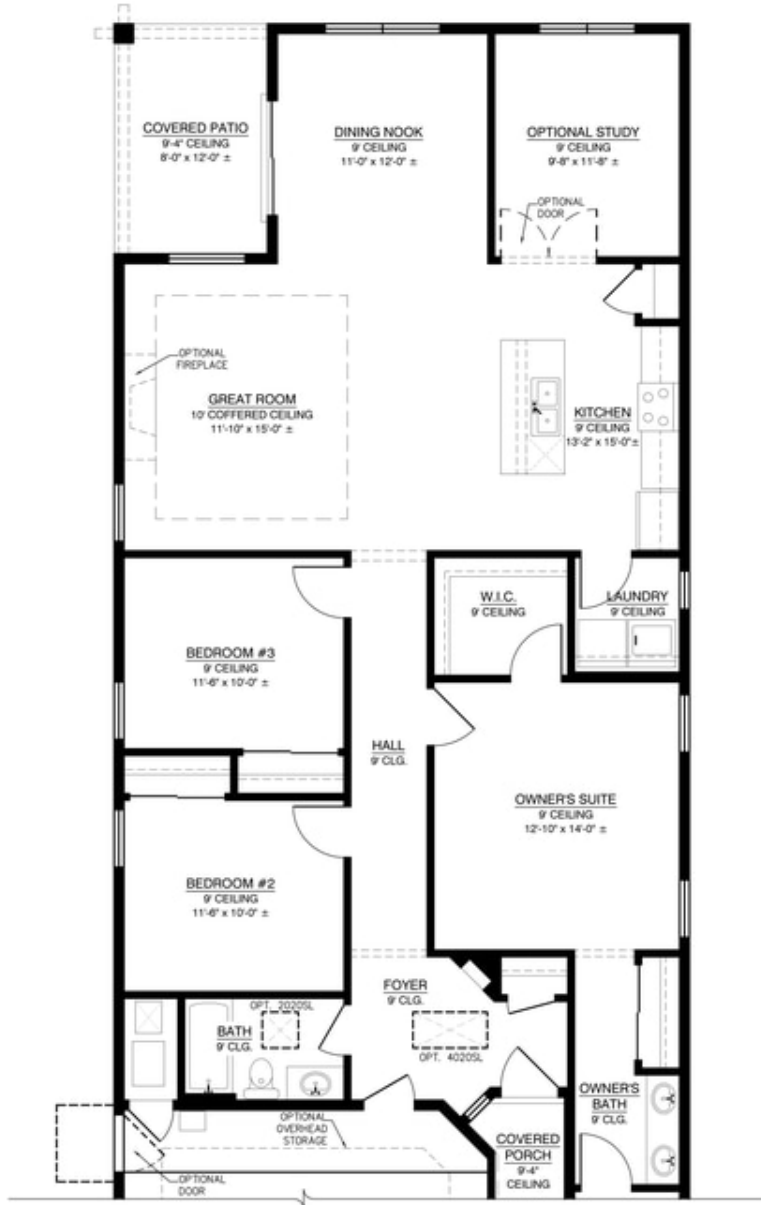
PARTIAL FLOOR PLAN OPTIONAL STUDY
