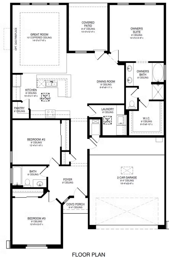
FLOOR PLAN
